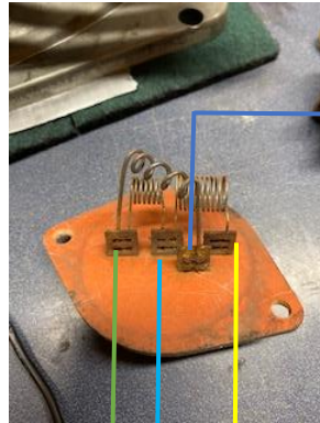
Blower Resistor
